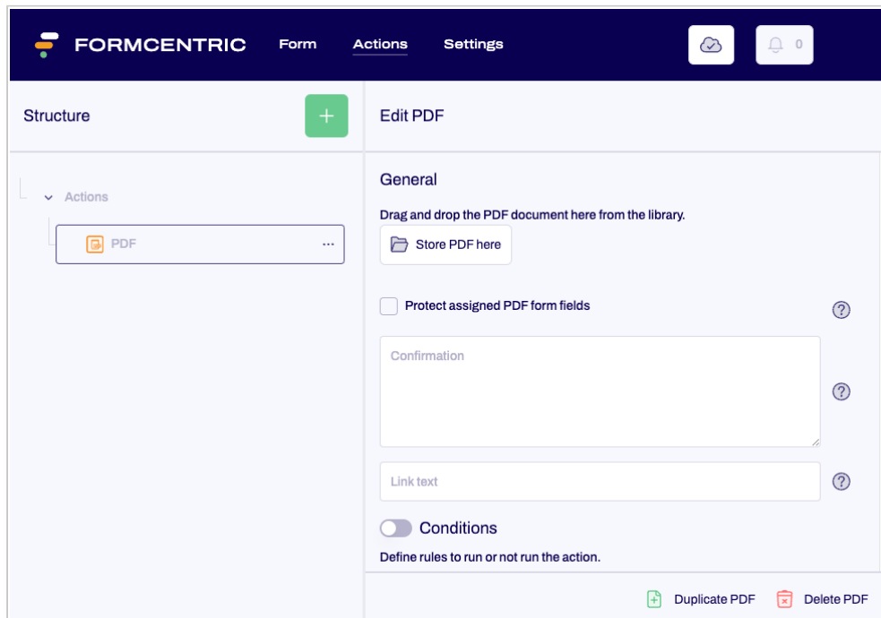
Figure 4.5. PDF action
