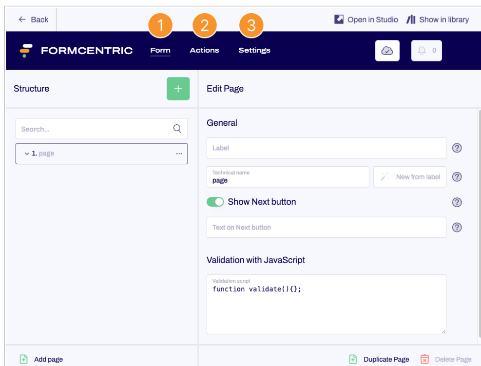
Figure 2.1. Editing interface
