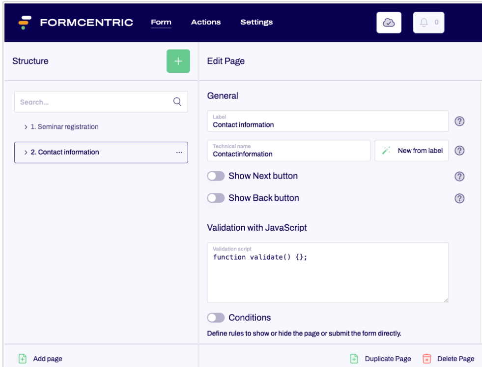
Figure 3.2. Page properties
