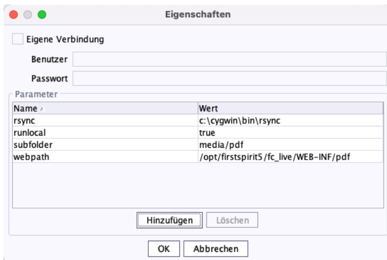
Figure 4.40. Sample configuration for the PDF action deployment script on a Windows server
