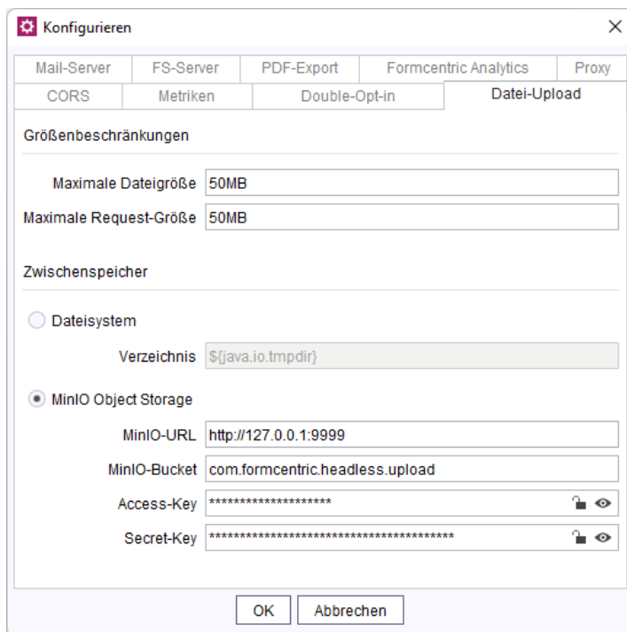
Figure 4.19. Configuring file uploads
