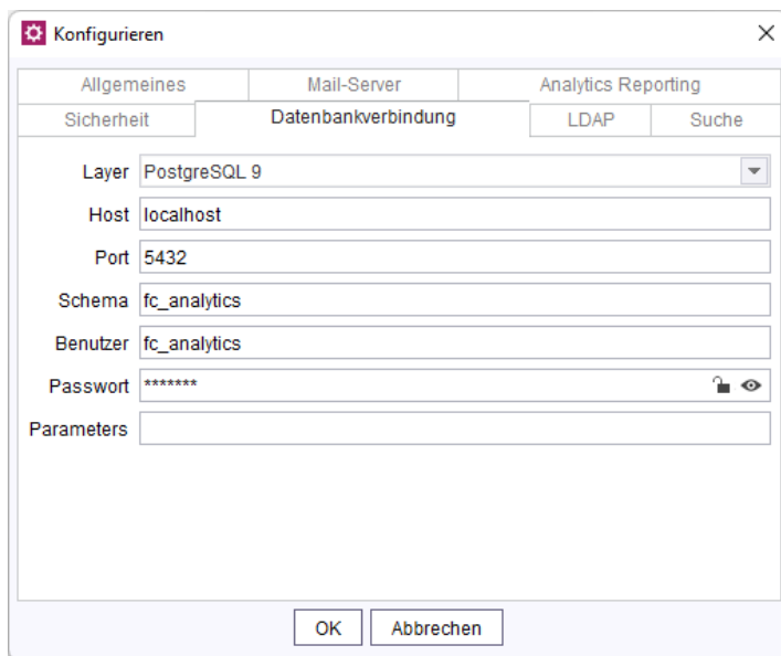
Figure 4.26. Configuring the Analytics Backend web application on the “Database connection” tab
