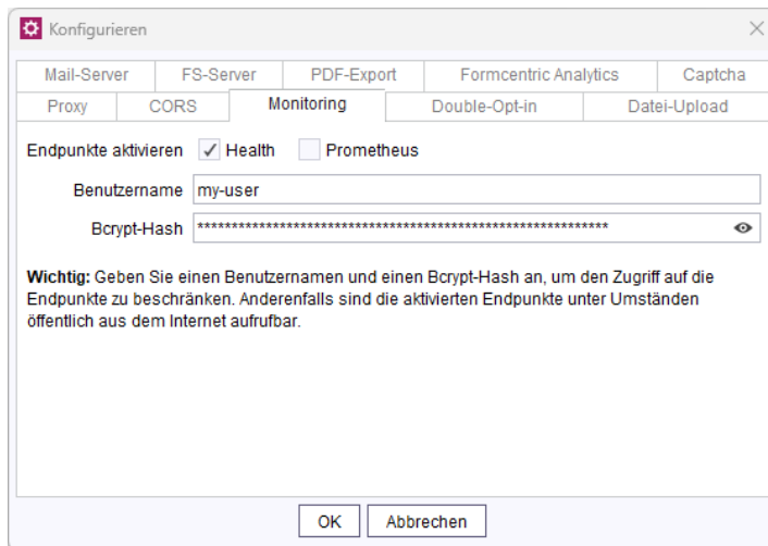
Figure 4.17. Configuring the credentials for displaying the metrics
